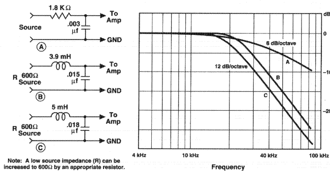
Fig. 3.5 RFI Filters
