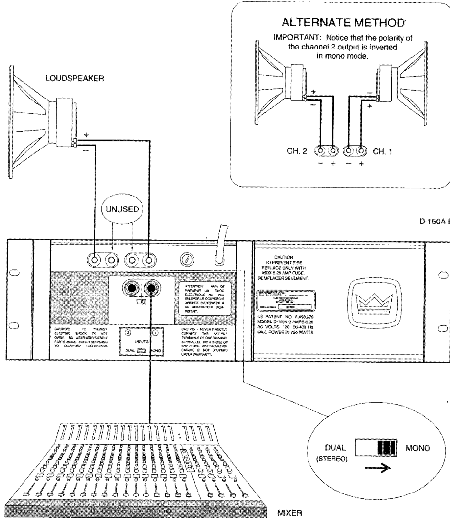
Fig. 3.3 Mono System Connection
