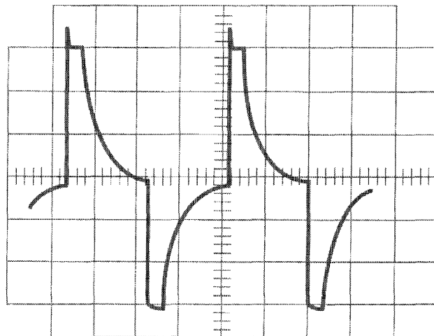
Figure 5.2 Differentiated Square Wave
