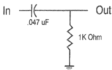
Figure 5.1 Differentiator Circuit
