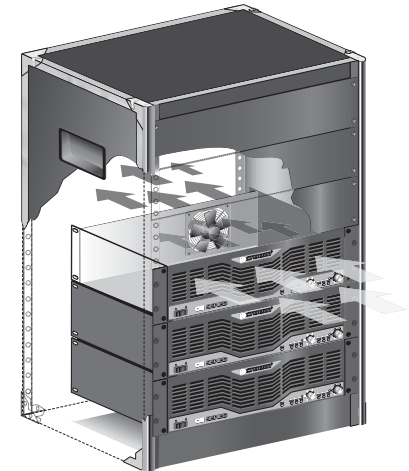
Figure 2.2 Airflow
