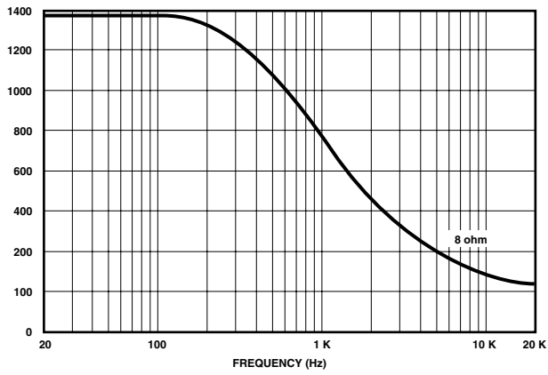
Fig. 6.8 Typical Damping Factor
